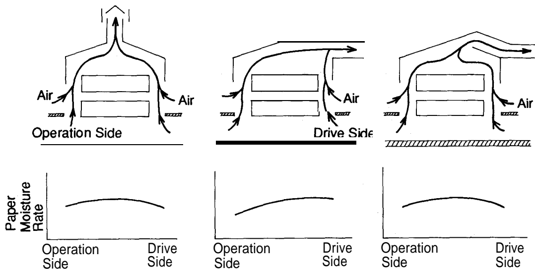
Figure 15 Air flow or paper moisture profile In different hood types
