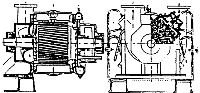
Drum type refiner
