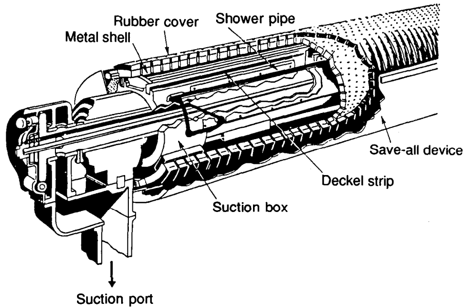
Figure 9 Suction roll
