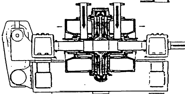
Disc type refiner
