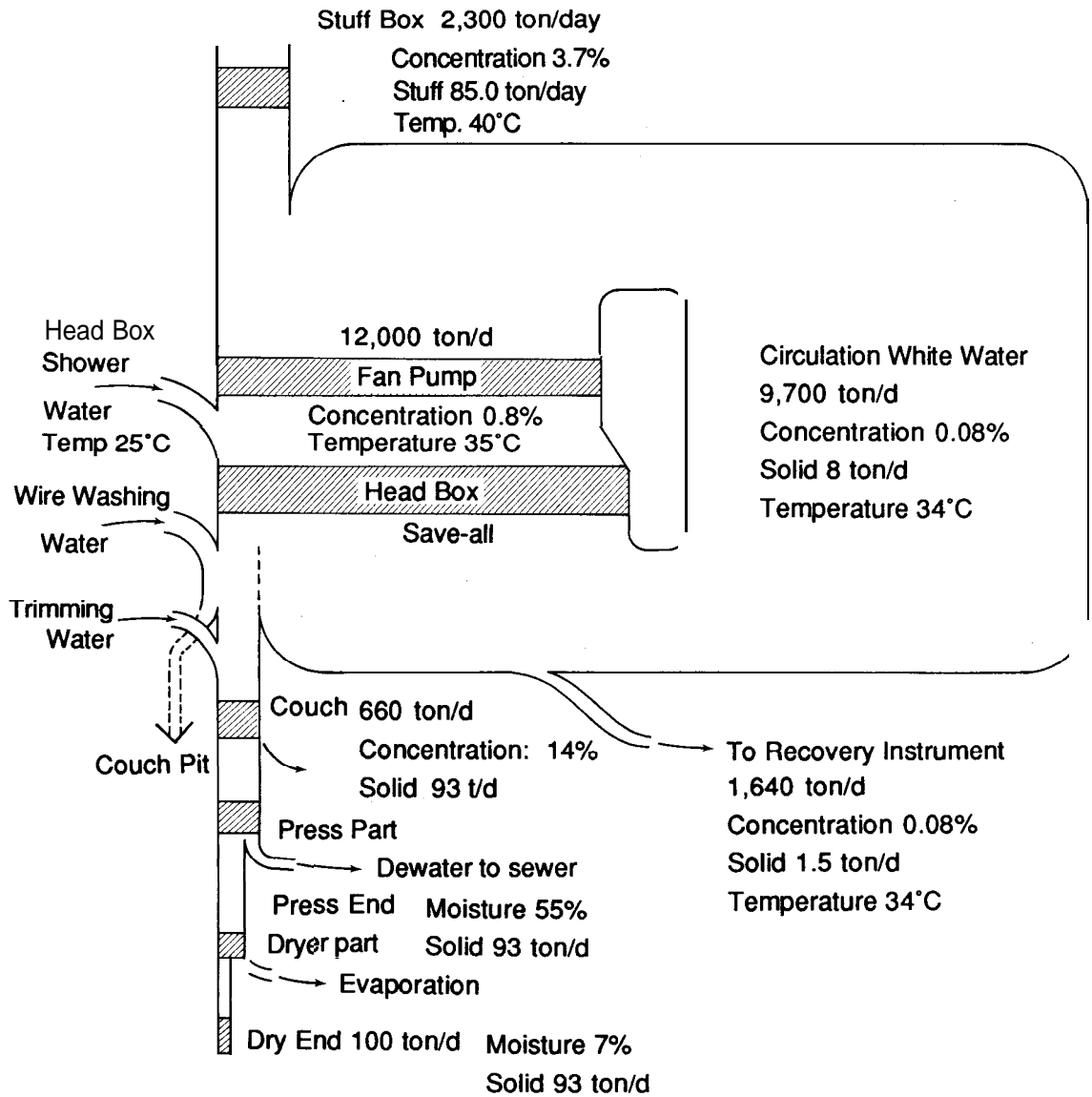
Figure 12 Typical water balance sheet of paper machine
