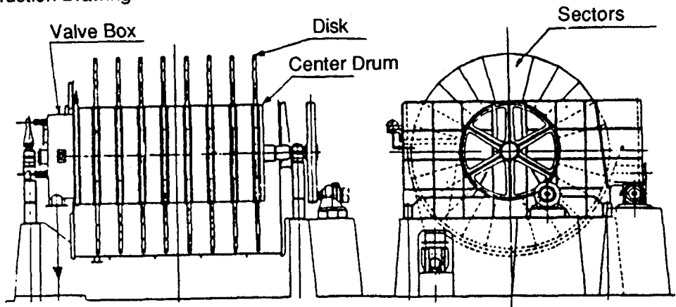
Figure 14 Polydiskfilter
