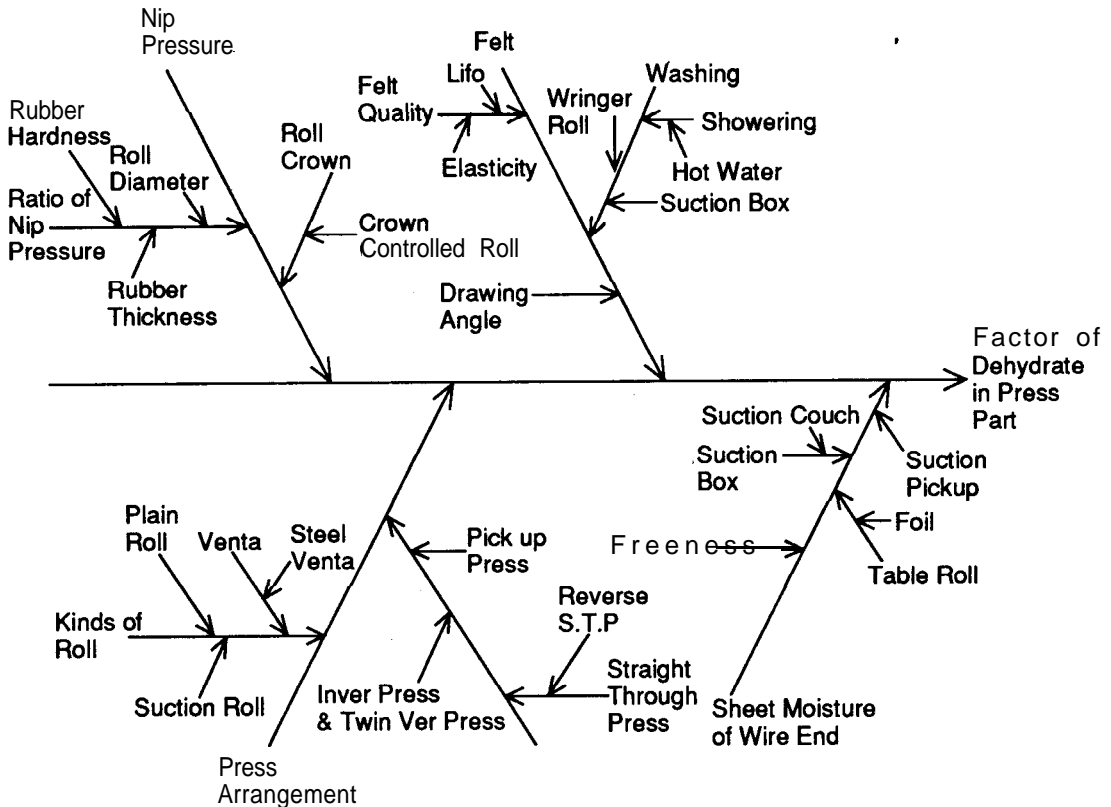
Figure 7 Cause and effect diagram of press dewatering
