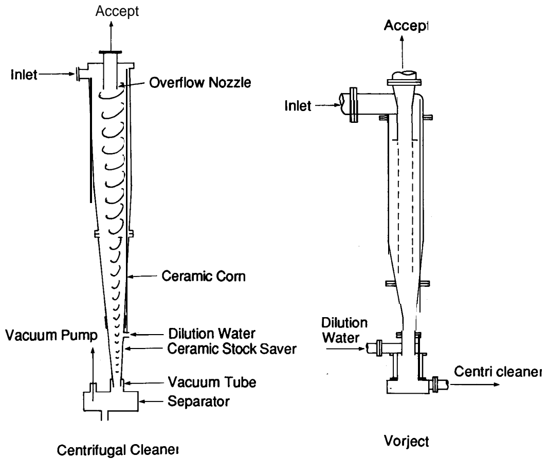
Figure 6 Centrifugal cleaner
