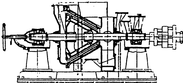
Drum type refiner
