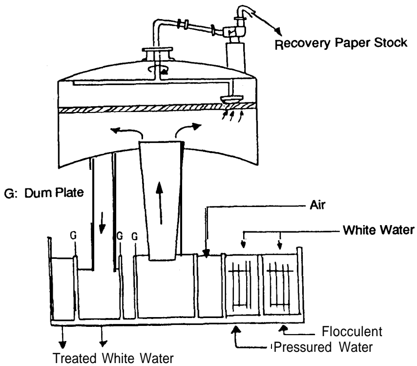
Figure 13 Adka save-all
