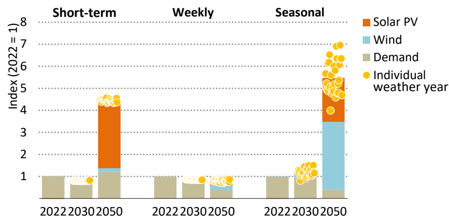
Figure 35. Evolution of flexibility needs and their drivers, 2022-2050
