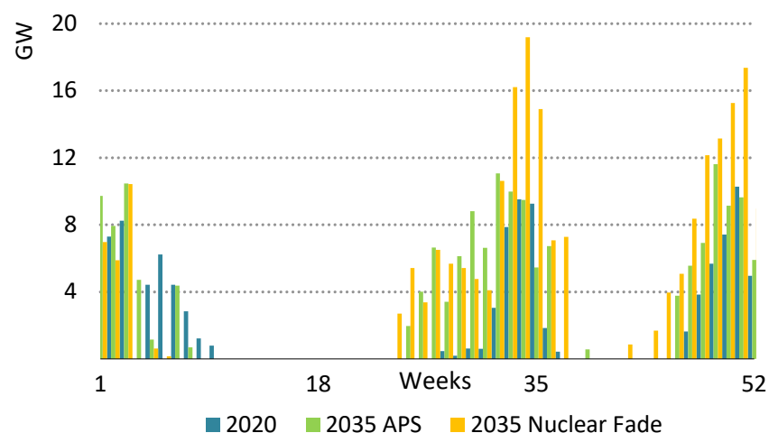
Figure 44. Seasonal flexibility needs in Korea by week in the Announced Pledges Scenario and Nuclear Fade case, 2020-2035
