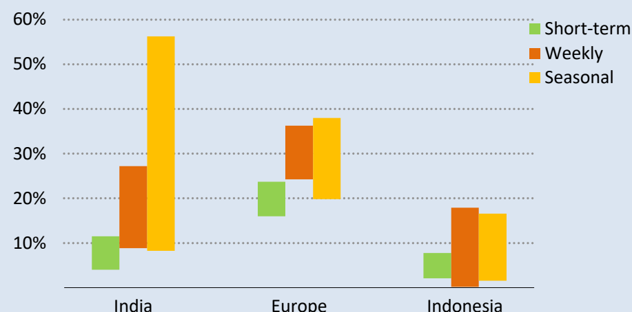
Figure 30. Increase of flexibility needs without interconnections or cross-border trade in the Announced Pledges Scenario, 2022-2050
