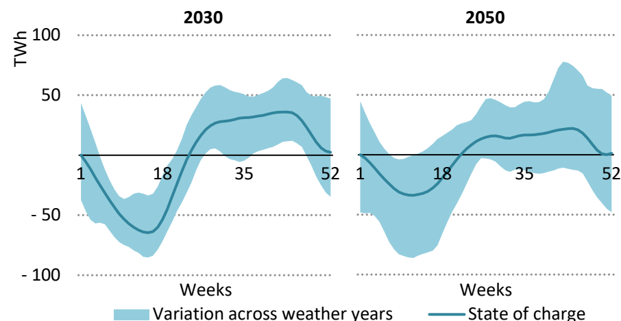
Figure 13. Variability of hydro seasonal storage across weather years, 2030 and 2050
