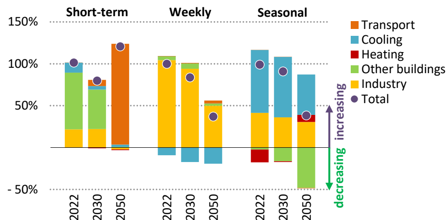
Figure 36. Contribution to flexibility needs by end-use, 2022-2050
