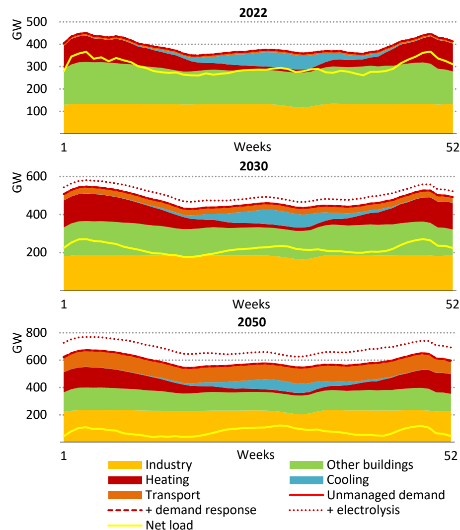
Figure 6. Average annual load curve by end-use, 2022-2050
