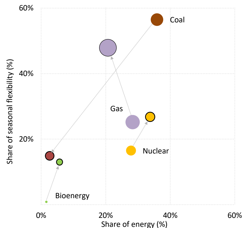
Figure 44. Share of energy and seasonal flexibility by source, Korea, Announced Pledges Scenario, 2020 and 2035
