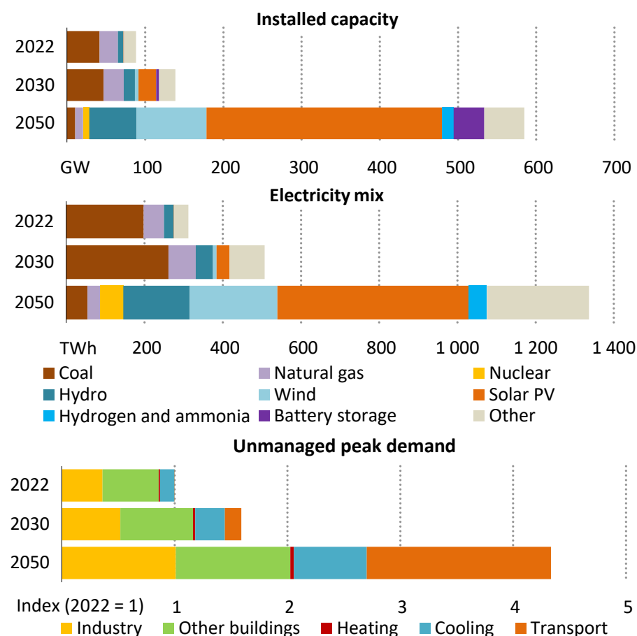
Figure 31. Evolution of installed capacity, generation mix and unmanaged peak demand, 2022-2050
