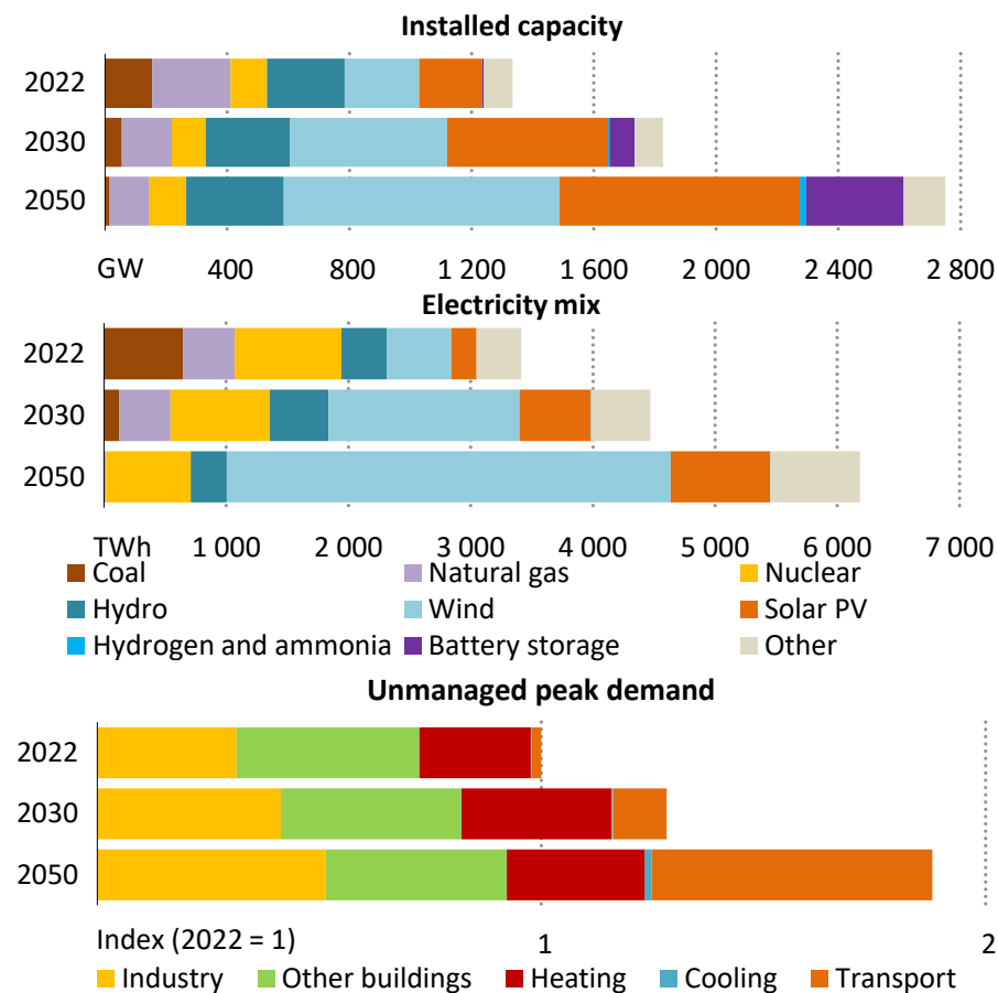
Figure 5. Evolution of installed capacity, generation mix and unmanaged peak demand, 2022-2050
