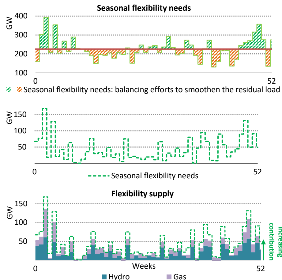
Figure 2. Profile of seasonal flexibility in Europe
