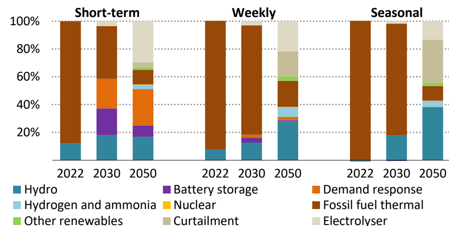
Figure 38. Flexibility supply by source, 2022-2050
