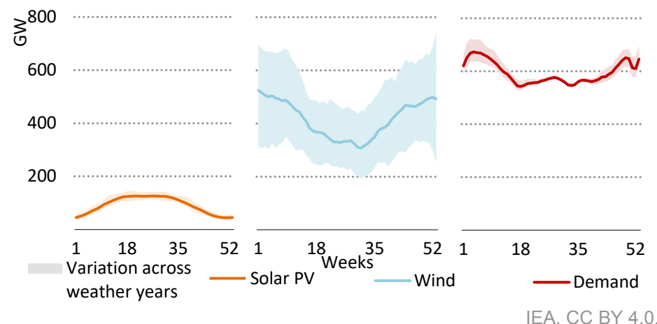
Figure 11. Variability across weather years in the Announced Pledges Scenario, 2050
