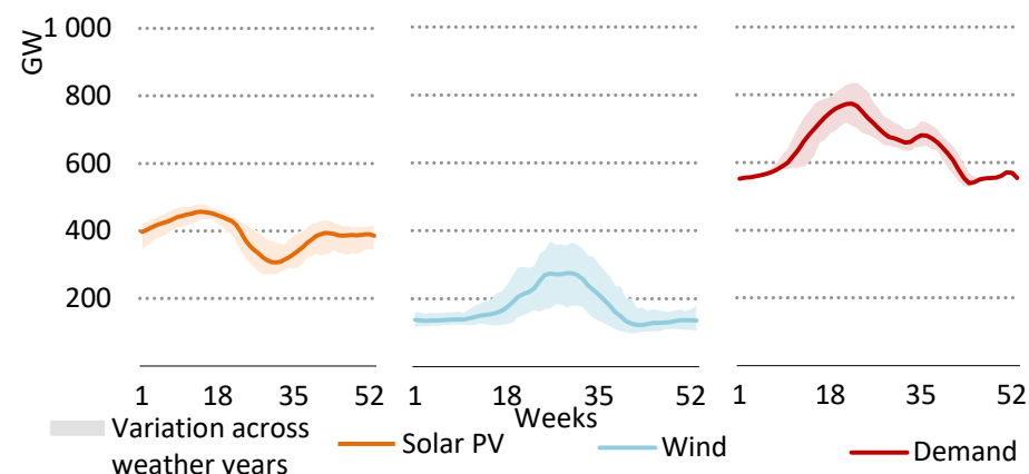
Figure 24. Variation across weather years in the Announced Pledges Scenario, 2050
