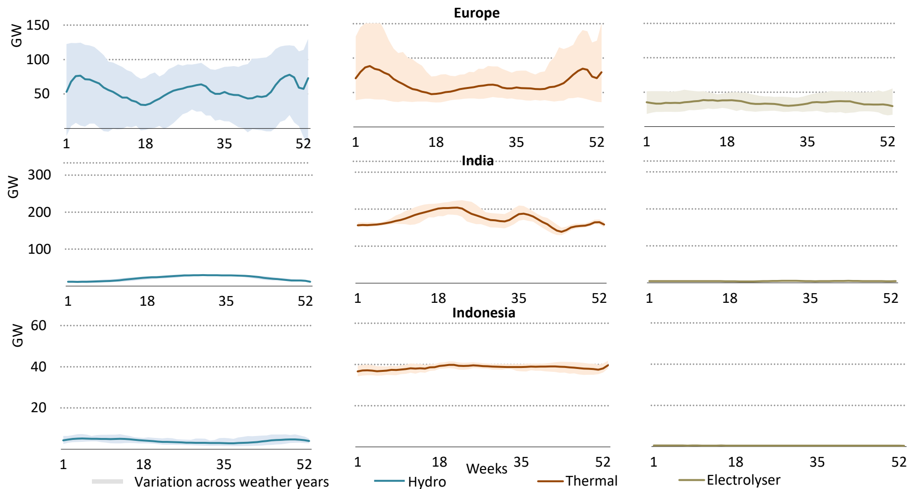
Figure 49. Variability across weather years, 2030
