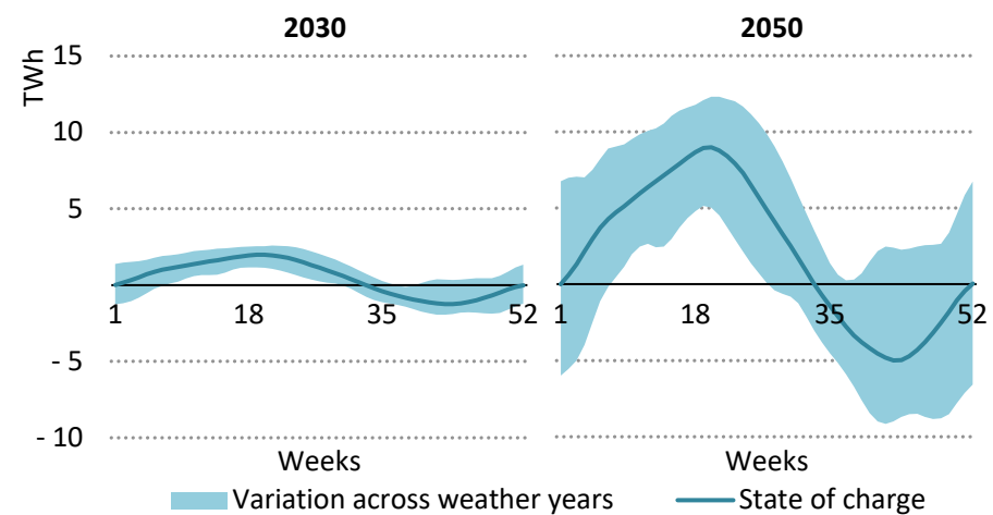
Figure 39. Variability of hydro seasonal storage across weather years, 2030 and 2050
