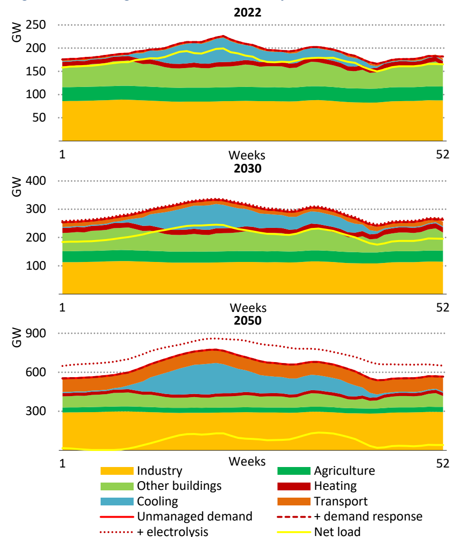
Figure 19. Average annual load curve by end-use, 2022-2050
