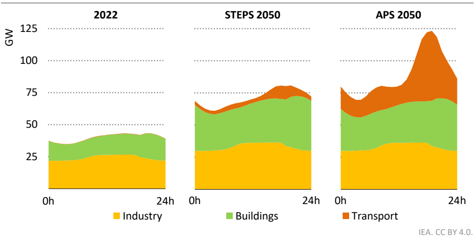
Figure 5.52 ▶ Average electricity daily load profile by scenario in Mexico
