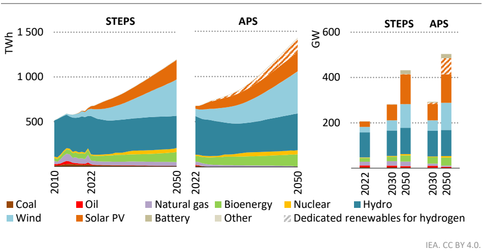
Figure 5.21 ▶ Electricity generation and capacity by fuel and scenario in Brazil
