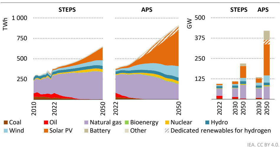
Figure 5.53 ▶ Electricity generation and capacity by fuel and scenario in Mexico
