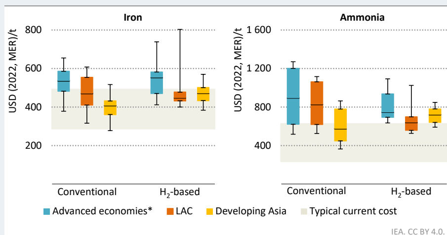
Figure 4.14 ▶ Levelised cost of production of iron and ammonia by process type in selected regions in the NZE Scenario, 2030
