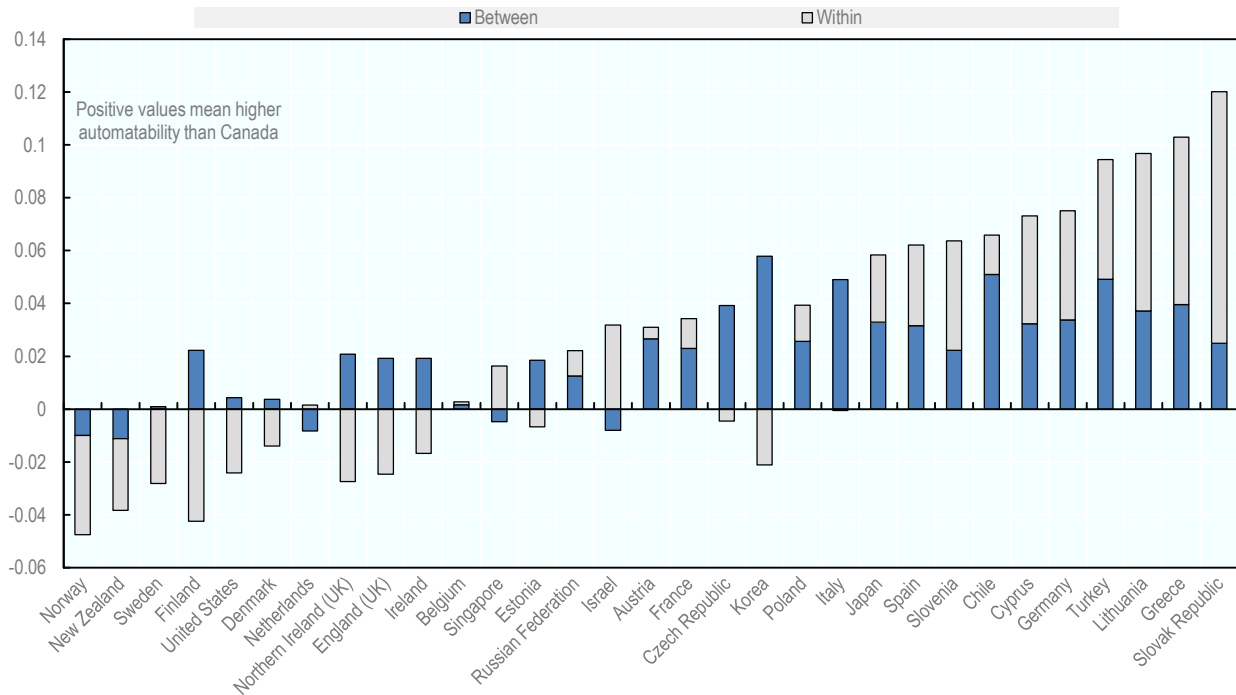
Figure 4.9. Decomposition of cross-country differences in the level of automatability along the industry dimension
