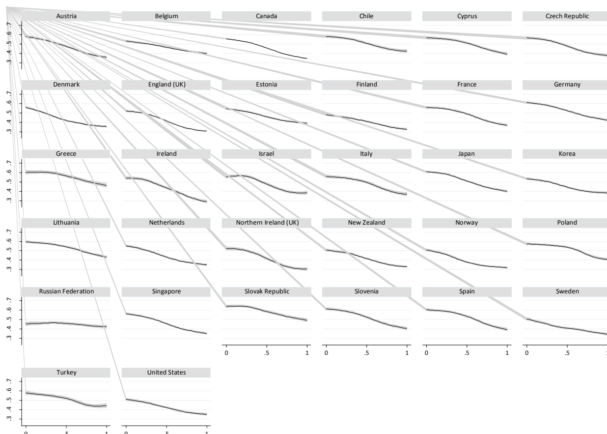
Figure 4.6. Automatability and earnings
